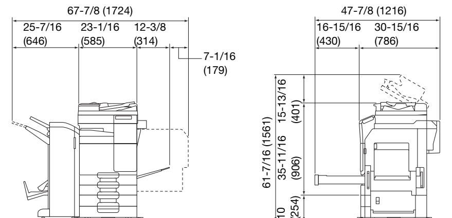
bizhub C287/C227 + DF-628 + PC-214 + MK-603 + RU-514 + FS-534 SD + MK-748 + CU-101
